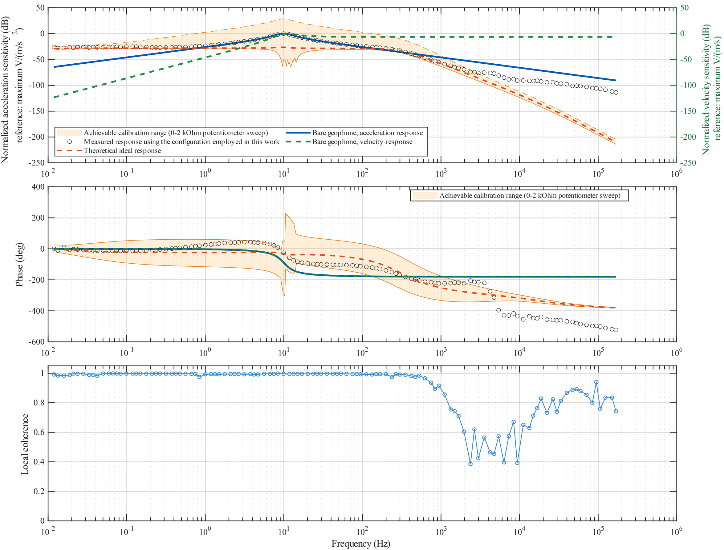
Complete GEO-to-ADC Chain: Measurement, Calibration Range, and Theoretical Response
